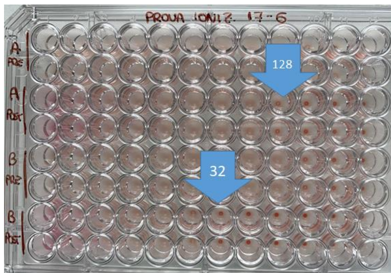
Figure 3b –Representative image of hemagglutination results
