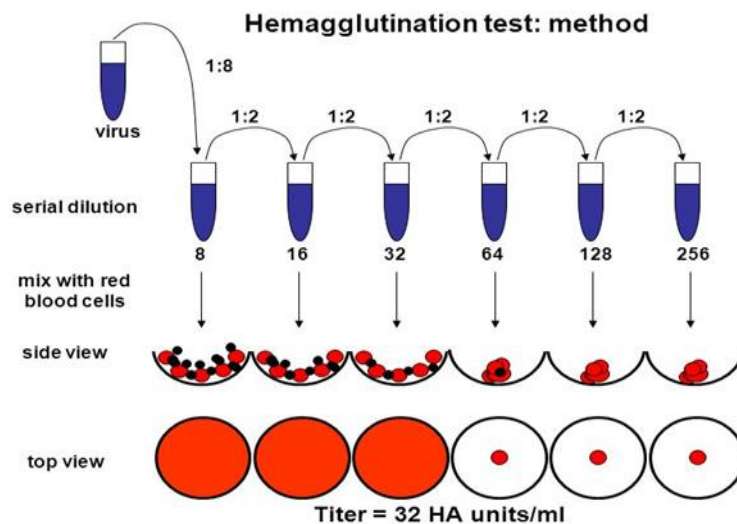
Figure 2a – Schematic representation of hemagglutination test
