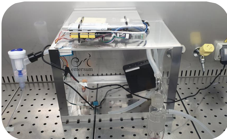
Figure 1 – Experimental system: Nebulization (Left), exposition (centre), biosampler collector (bottom)
